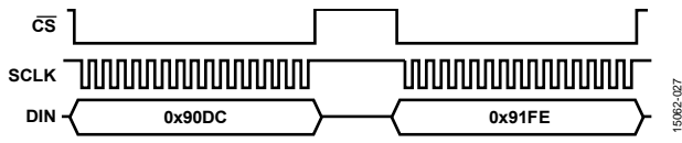
Figure 27. SPI Sequence for Writing 0xFEDC to XG_BIAS_LOW
