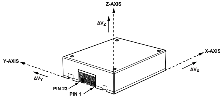
Figure 36. Delta Velocity Axis and Polarity Assignments
