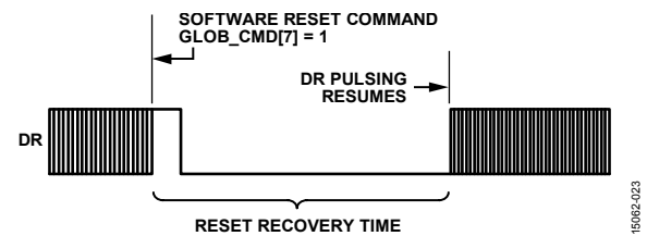
Figure 23. Data Ready Response During Reset (Register GLOB_CMD, Bit 7 = 1) Recovery
