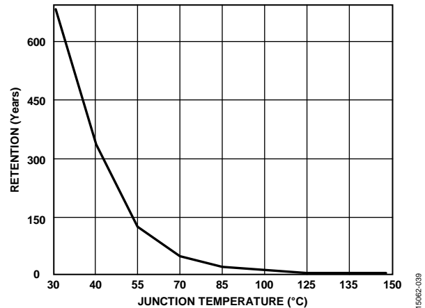
Figure 39. Flash Memory Retention
