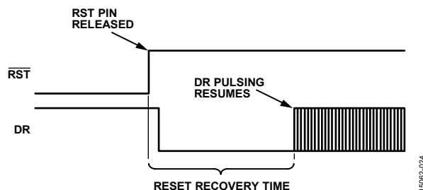
Figure 24. Data Ready Response During Reset ( \bar{RST} = 0 ) Recovery
