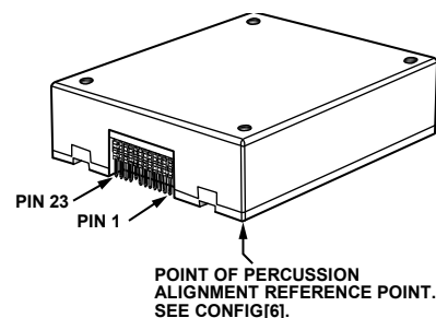
Figure 40. Point of Percussion Reference Point
