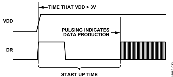
Figure 22. Data Ready Response During Startup
